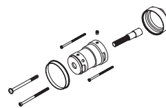
RP74785 Available Extension Kit
